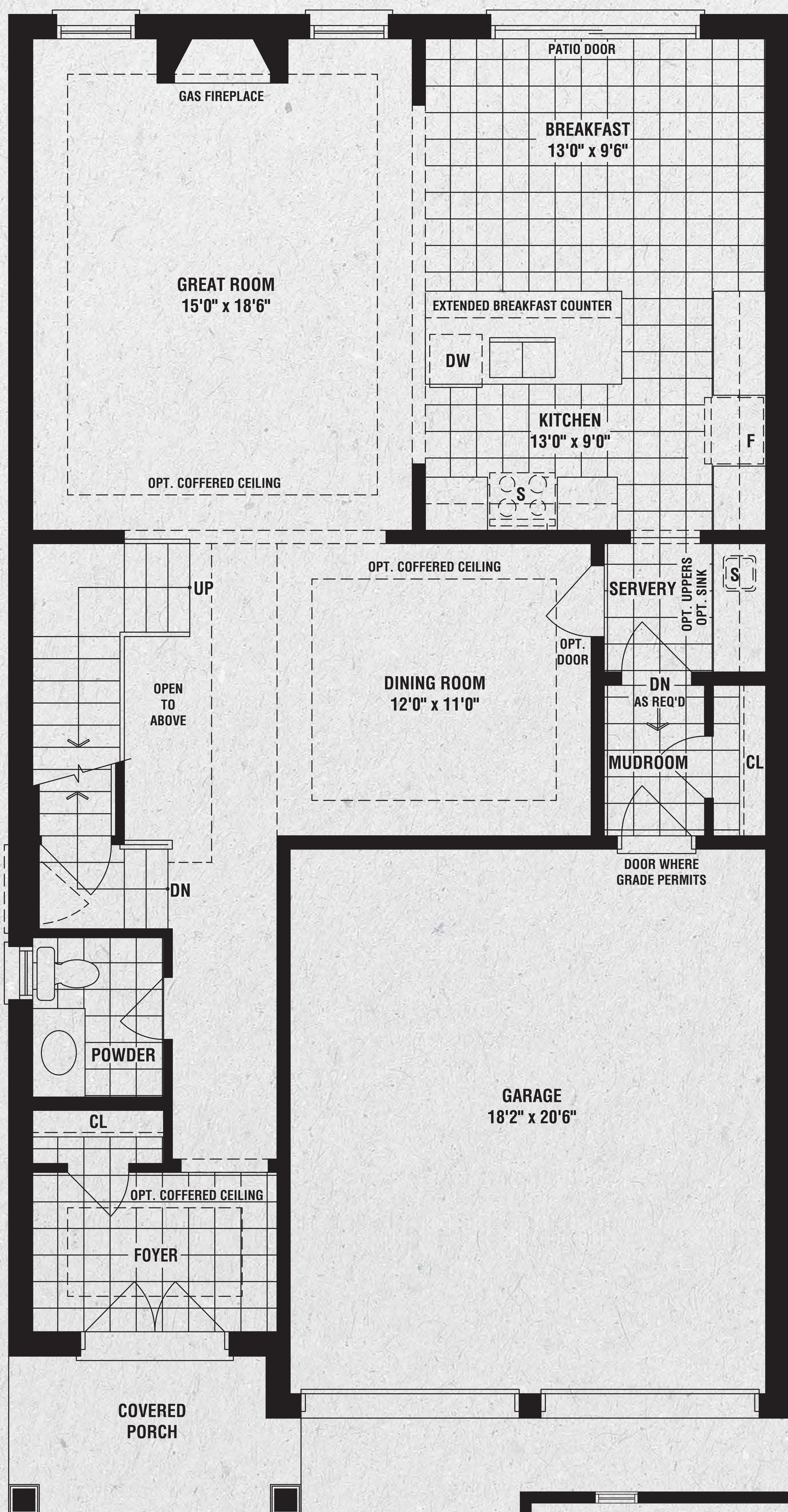
GROUND FLOOR ELEV. 'A'
